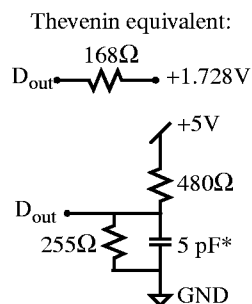
Figure C: Output load for t_{CLZ} , t_{CHZ} , t_{OLZ} , t_{OHZ} , t_{WZ} , t_{OW}
